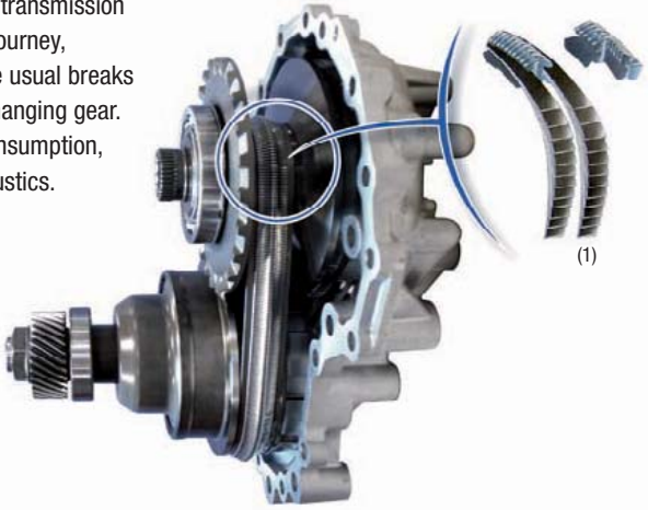
(1) 2 pulleys of varying diameters in the mechanism's housing held together by a steel belt.
